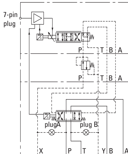
Detailed Symbol
