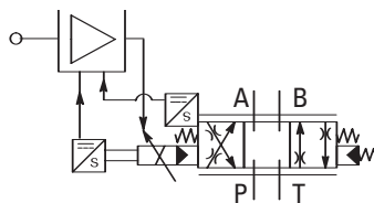
Simplified Symbol
